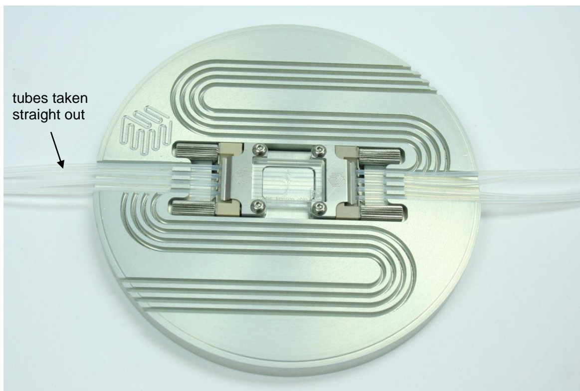
Chip heating without pre-heating and post-heating of liquids
