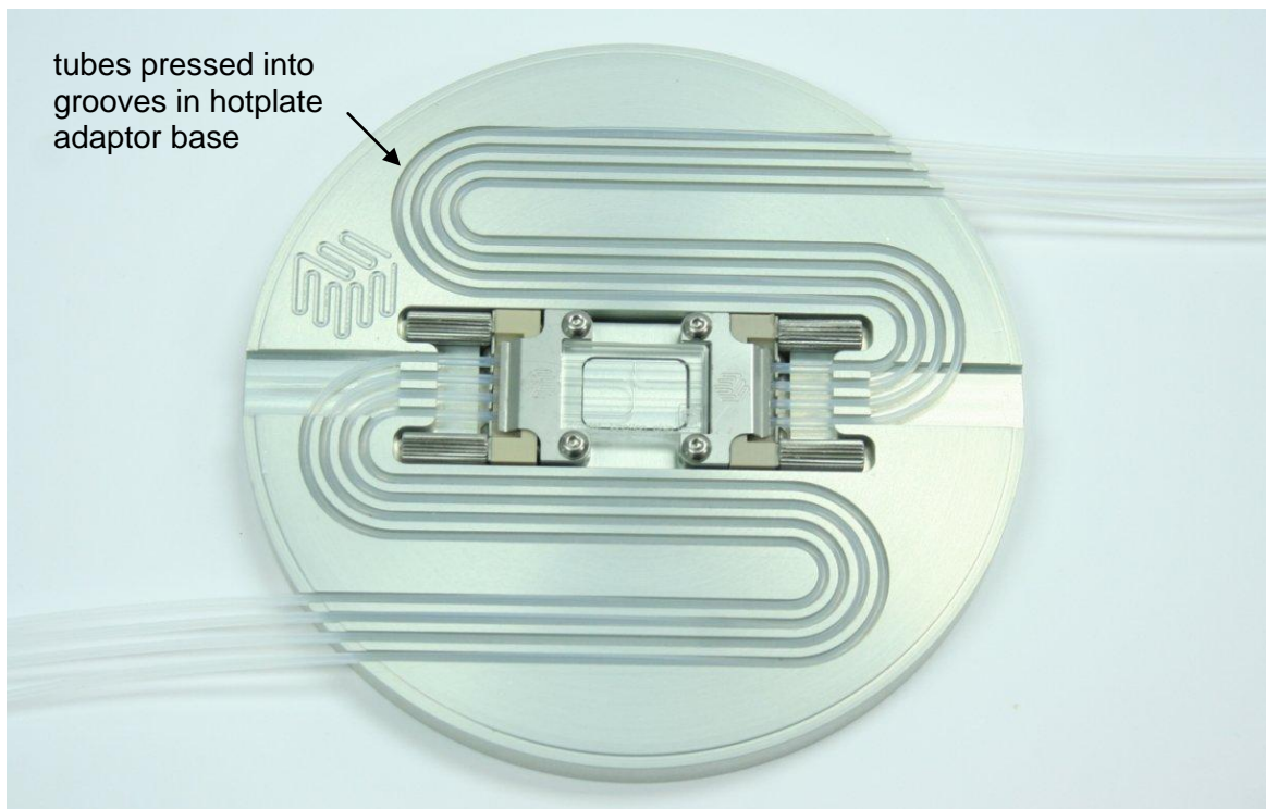
Chip heating with pre-heating and post-heating of liquids
